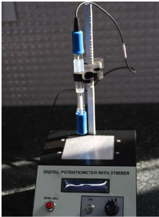
Digital Potentiometer
